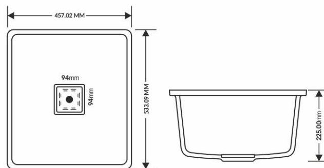
DIMENSION SIZE
