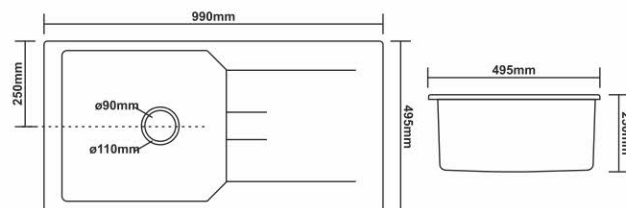
DIMENSION SIZE
