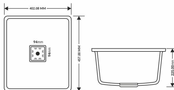
DIMENSION SIZE
